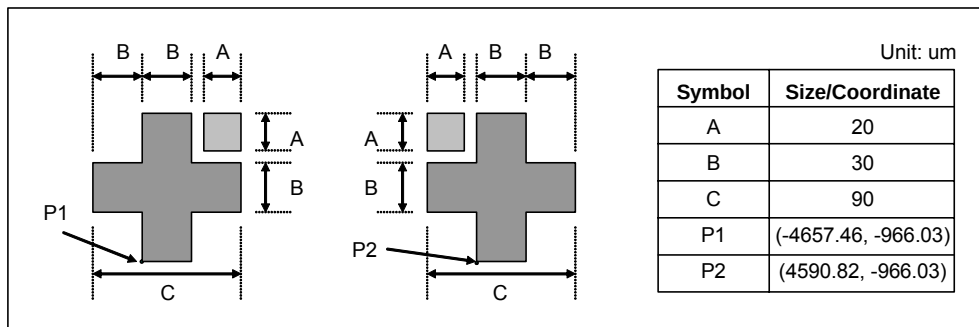
Figure 8-2 : Fixed Point Dimension
