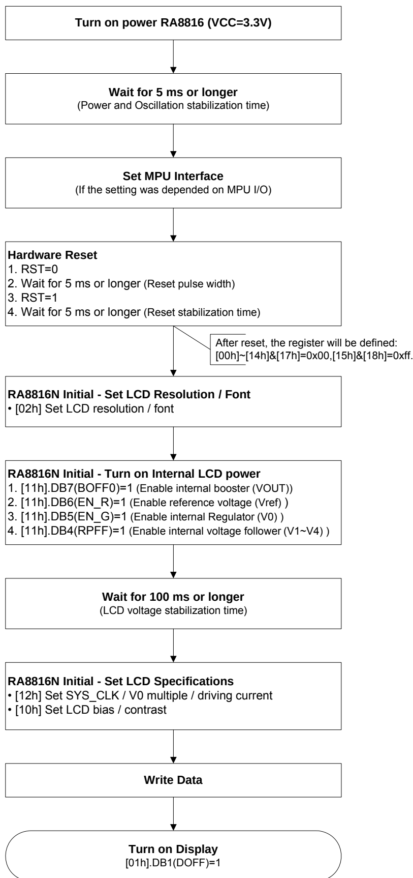
Figure 6-34 : Power On Sequence
