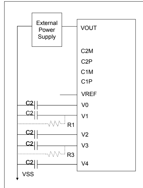
Figure 6-24 : External VOUT
