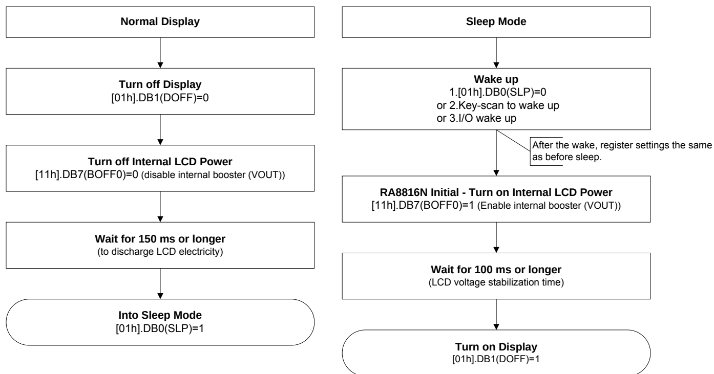
Figure 6-36 : Sleep/Wake up Sequence
