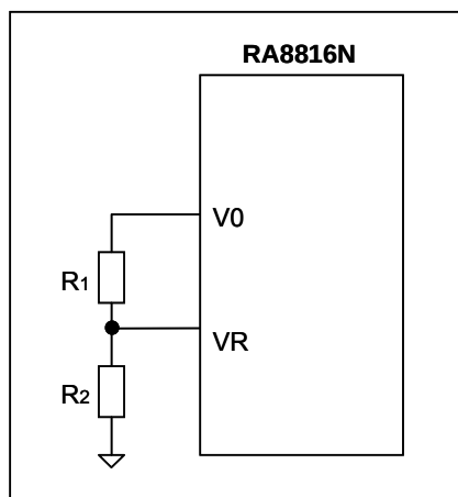
Figure 6-26 : Use External Resistor Divider
