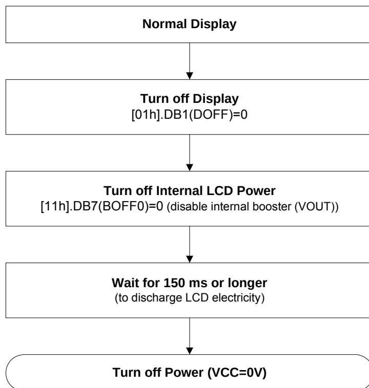
Figure 6-35 : Power Off Sequence
