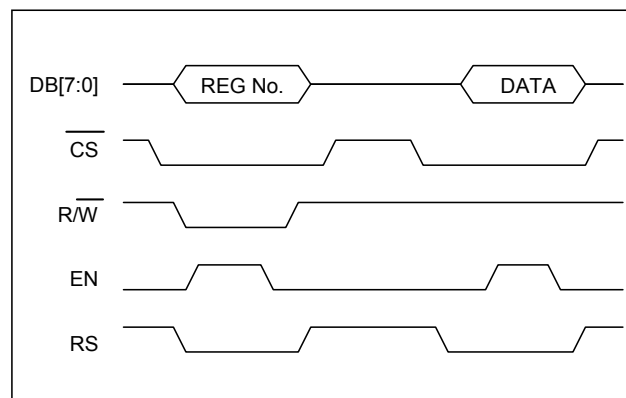
Figure 6-9 : Register Read on 6800 (8-bit) I/F
