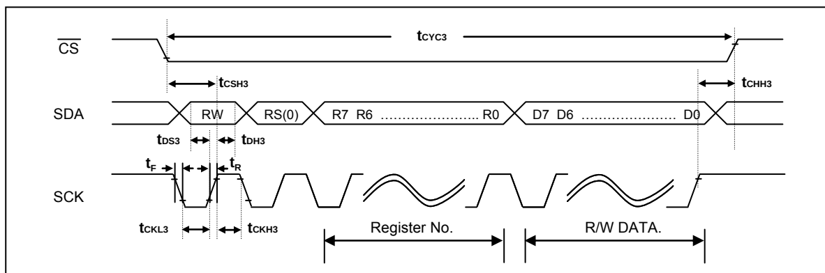
Figure 9-3 : 3-Wire Timing
