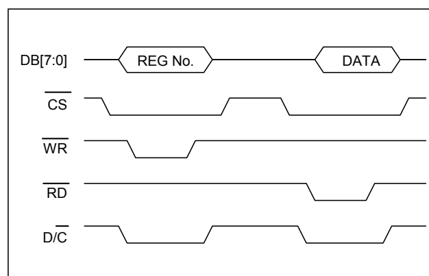
Figure 6-7 : Register Read on 8080 (8-bit) I/F
