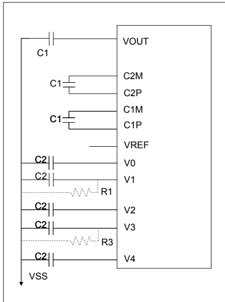
Figure 6-23 : Internal VOUT (3*VDD)
