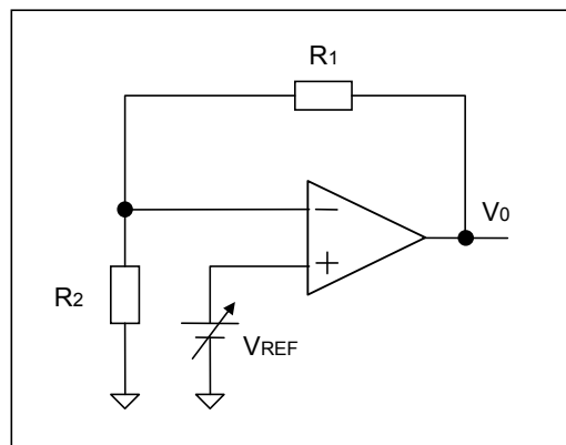
Figure 6-25 : Voltage Regulator
